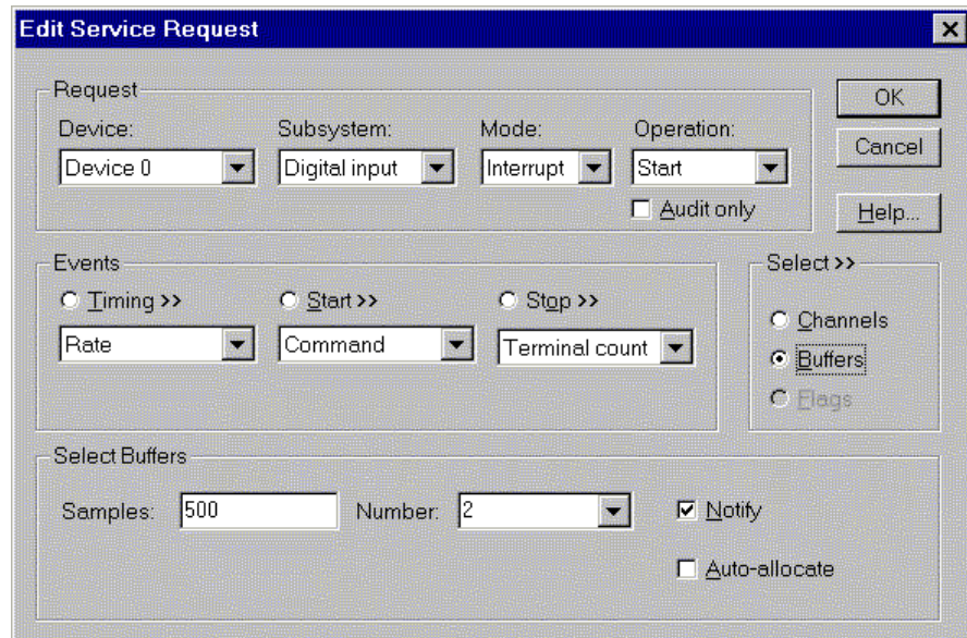
How to set up the KPCMCIA-8AO Series to read digital samples using data buffers
